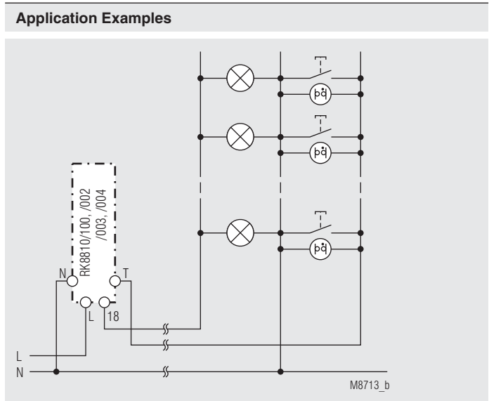
3-wire circuit N on push button
