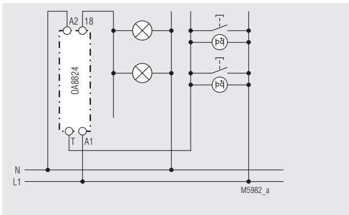
OA 8824 4-wire circuit (cannot be reswitched)
