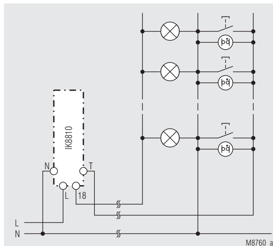
3-wire circuit N on push button
