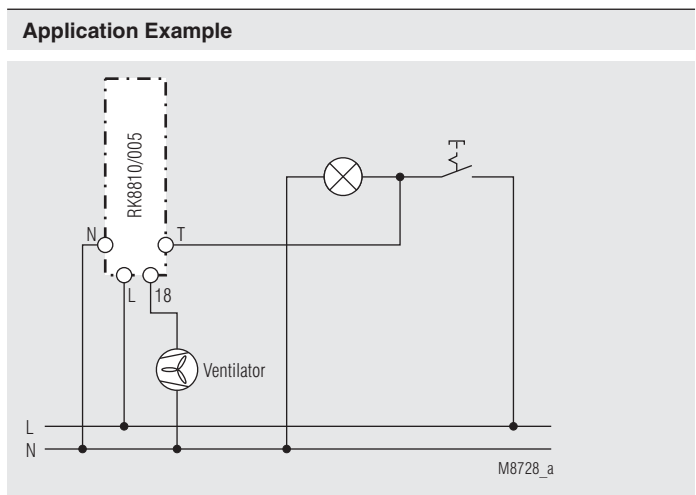
circuit L on push button
