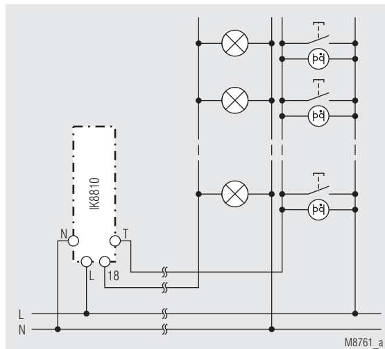
4-wire circuit L on push button
