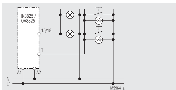
IK 8825 / OA 8825 4-wire circuit (reswitching possible)
