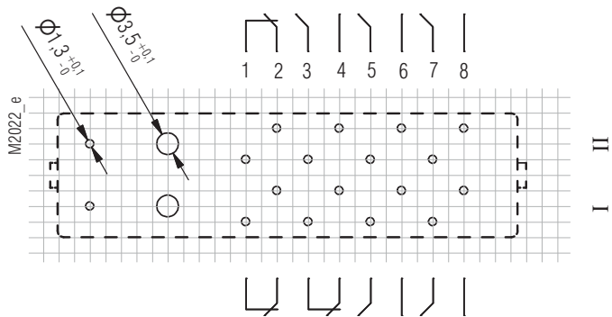
Pin arrangement OA5603.58 5NO/3NC
