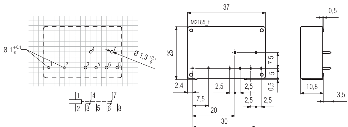
Drilling plan (solder side)
