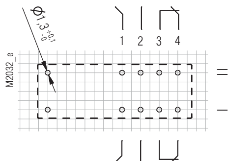
Pin arrangements OA 5611.52/...L5 2NO / 2NC
