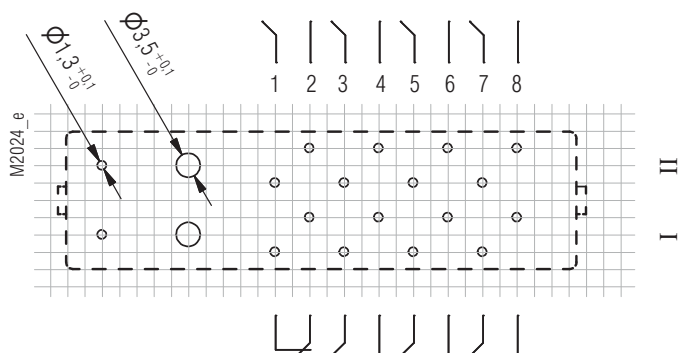
Pin arrangement OA5603.63 7NO/1NC
