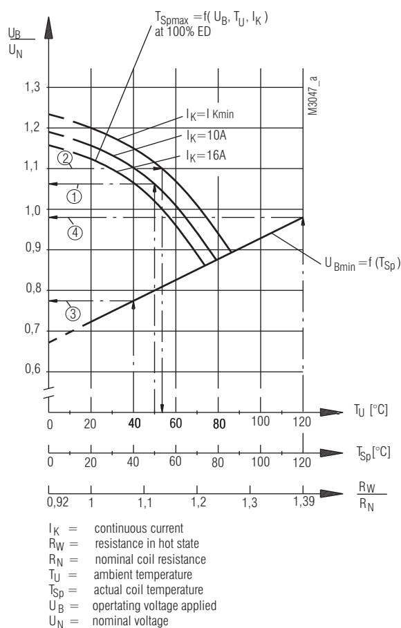
Operating voltage limit curve
