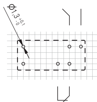
Pin configuration standard
