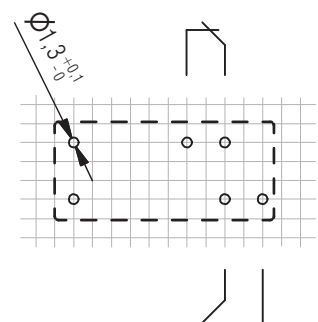
Pin configuration reverse
