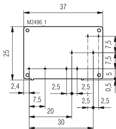
Drilling plan (solder side)
