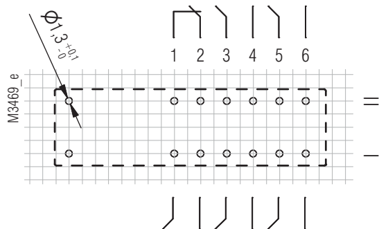
Pin arrangement OA 5612.54/...S4 4NO / 2NC
