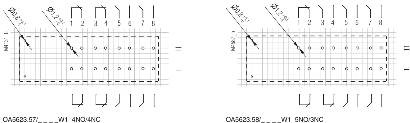
Pin configuration W1 Drilling plan (solder side)
