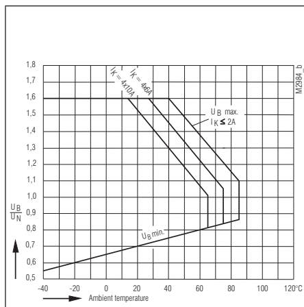
Operating voltage limit curve OA 5602
