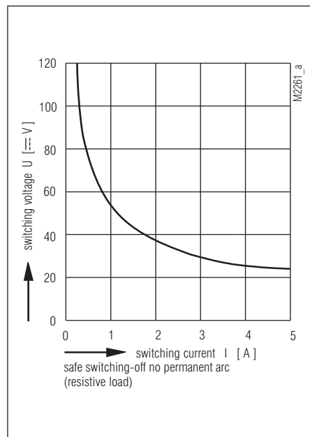
Arc limit curve at t_u = 20^\circ\text{C} for OW 5691 and OW 5699
