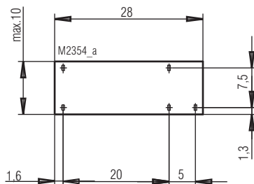
Drilling plan (solder side)
