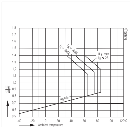
Operating voltage limit curve OA 5611
