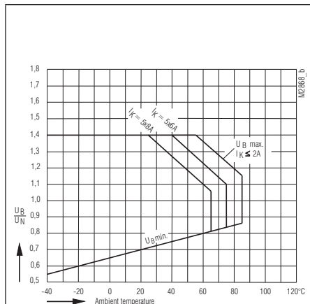
Operating voltage limit curve OA 5612
