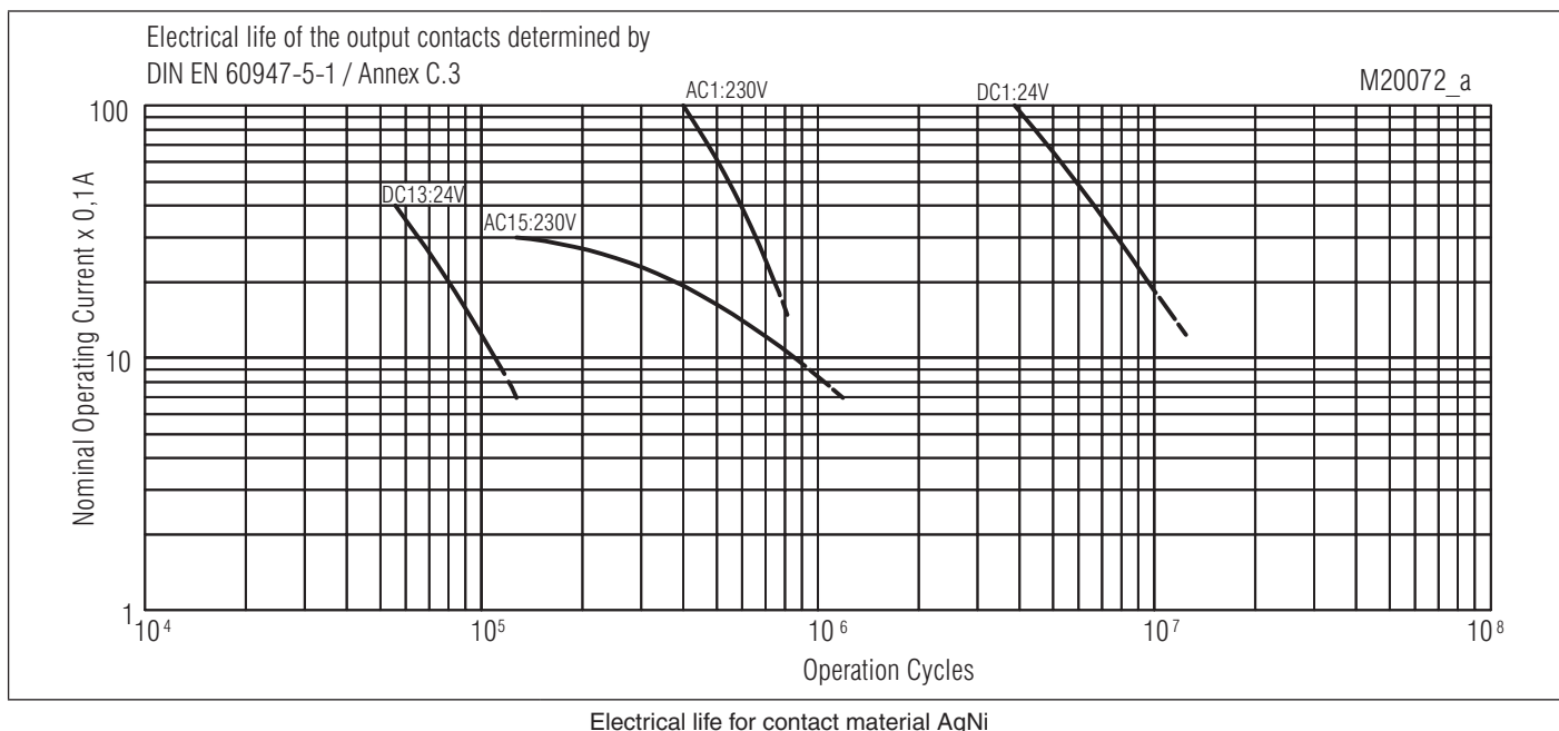
Electrical life for contact material AgNi
