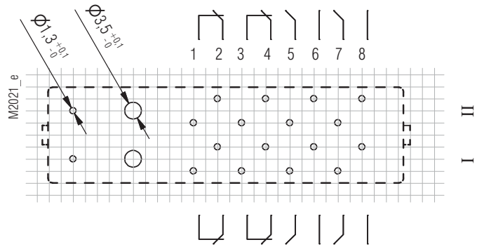
Pin arrangement OA5603.57 4NO/4NC
