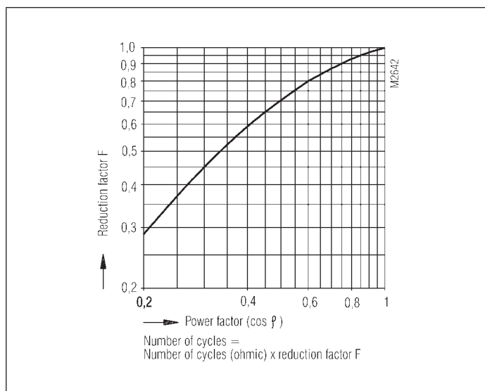
Reduction factor for inductive loads
