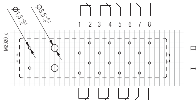
Pin arrangement OA5603.56 3NO/5NC
