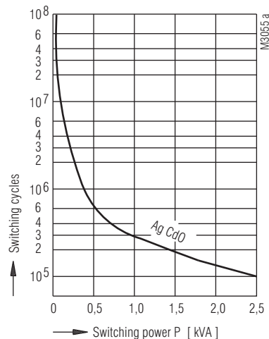
Contact service life OA 5690.11 10 A - model
