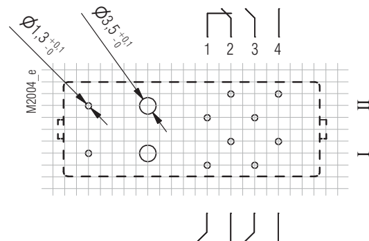
Pin arrangement OA5601.48 3NO/1NC
