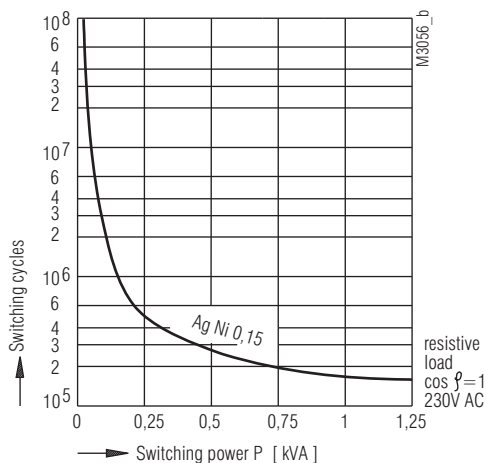
Contact service life OA 5690.11 5 A - model
