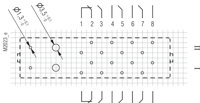
Pin arrangement OA5603.59 6NO/2NC
