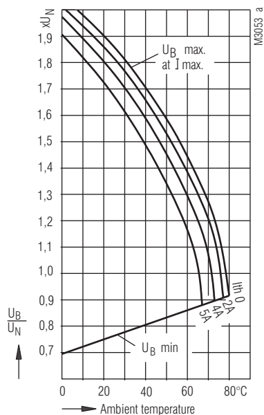
Operating voltage limit curve OA 5690.11 5 A - model
