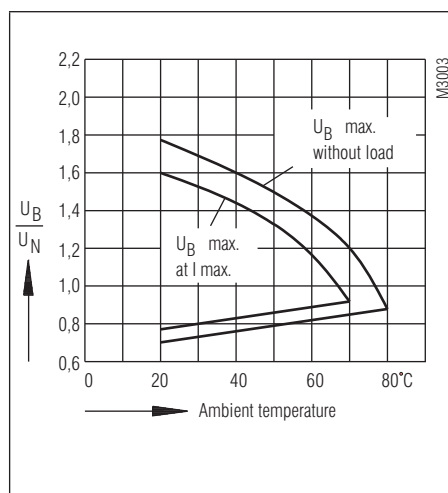
Operating voltage limit curve
