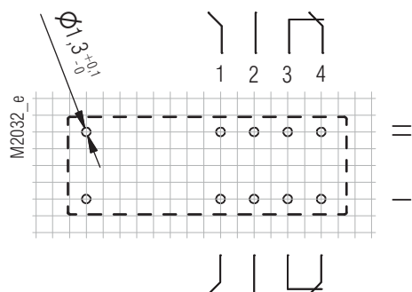
Pin arrangement OA 5611.52/...L5 2NO / 2NC
