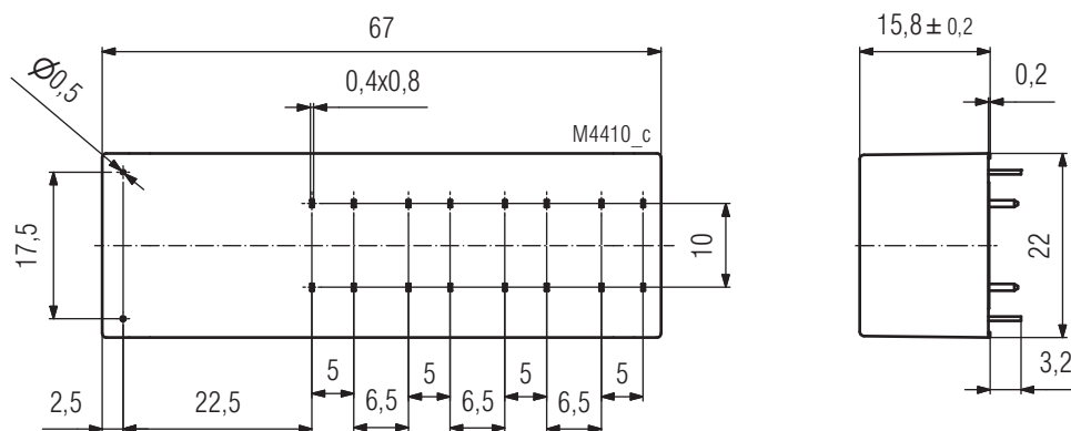
Pin configuration W1 Drilling plan (solder side)
