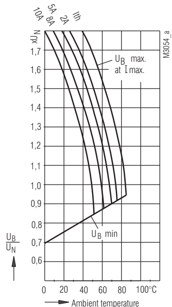
Operating voltage limit curve OA 5690.11 10 A - model
