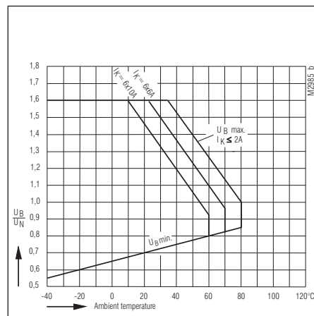
Operating voltage limit curve OA 5603
