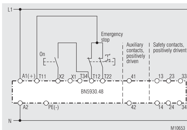
Two-channel emergency stop circuit Suited up to SIL3, Performance Level e, Cat. 4
