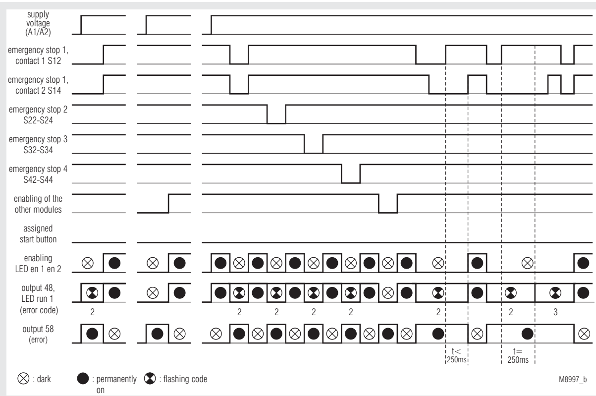
4 Emergency stop, Autostart, only enabling when all the other modules are enabled; function: 2
