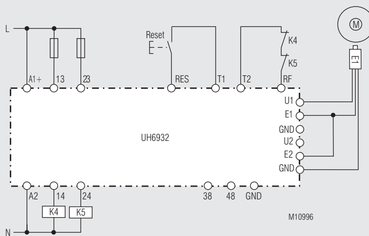
Connection with a proximity sensor, Suited up to SIL 2, Performance Level c, Cat. 2 (to achieve Cat. 2 the safety function has to be tested on a regular base)
