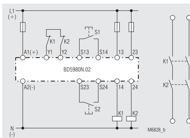
Two-hand control with contact reinforcement via external forcibly guided contactors. Suited up to SIL1, Performance Level c, Cat. 1
