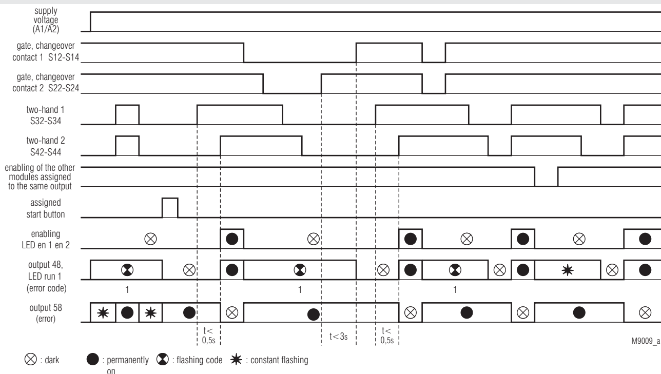
1 Safety gate, 1 two-hand control type IIIC; function: 8
