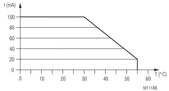
Continuous current limit curve semiconductor outputs
