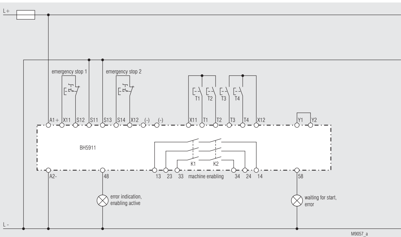
2 Emergency stop, single-channel; setting: 1, 5 or 9
