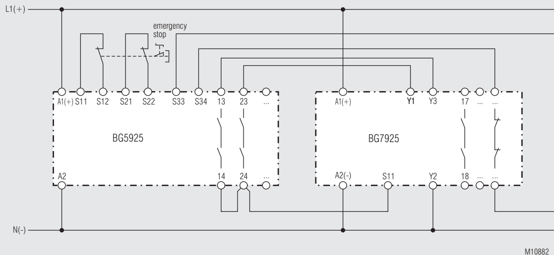
Versions with auxiliary voltage. Seperate control of 2 timing circuits with internal voltage S11 (+). Suited up to SIL2 Performance Level d, Cat. 3
