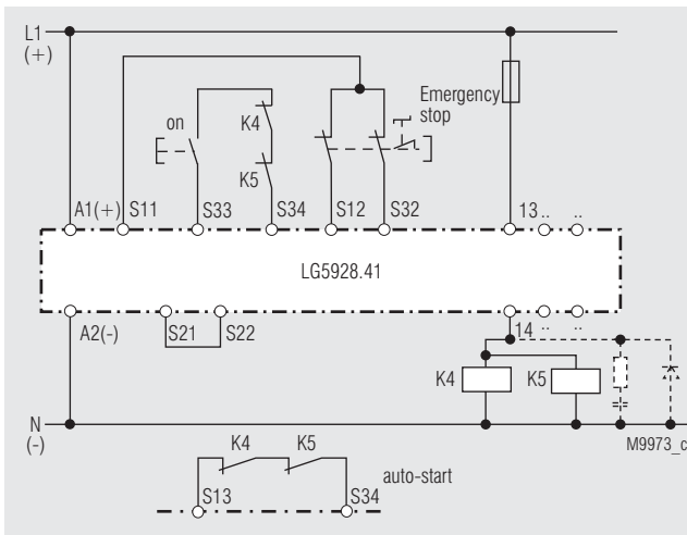
Contact reinforcement by external contactors controlled by one contact path. S33 - S34 must stay open on auto start. Suited up to SIL3, Performance Level e, Cat 4, if the external contactors are in the same cabinet and the wiring is short circuit and crossfault prove.
