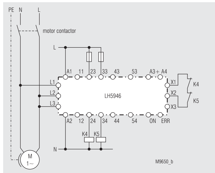
With single-phase motor; suitable up to SIL3, Performance Level e, Cat. 4
