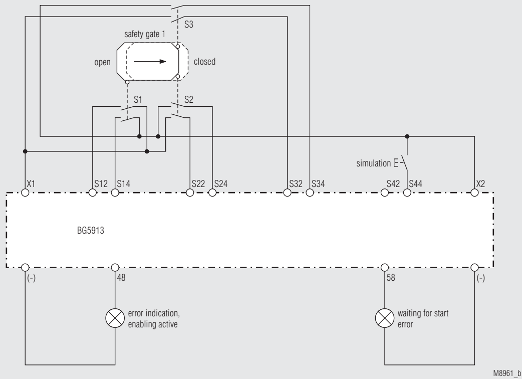
1 safete gate with 3 twin contacts, manual start (plastic injection moulding machines); function: 7
