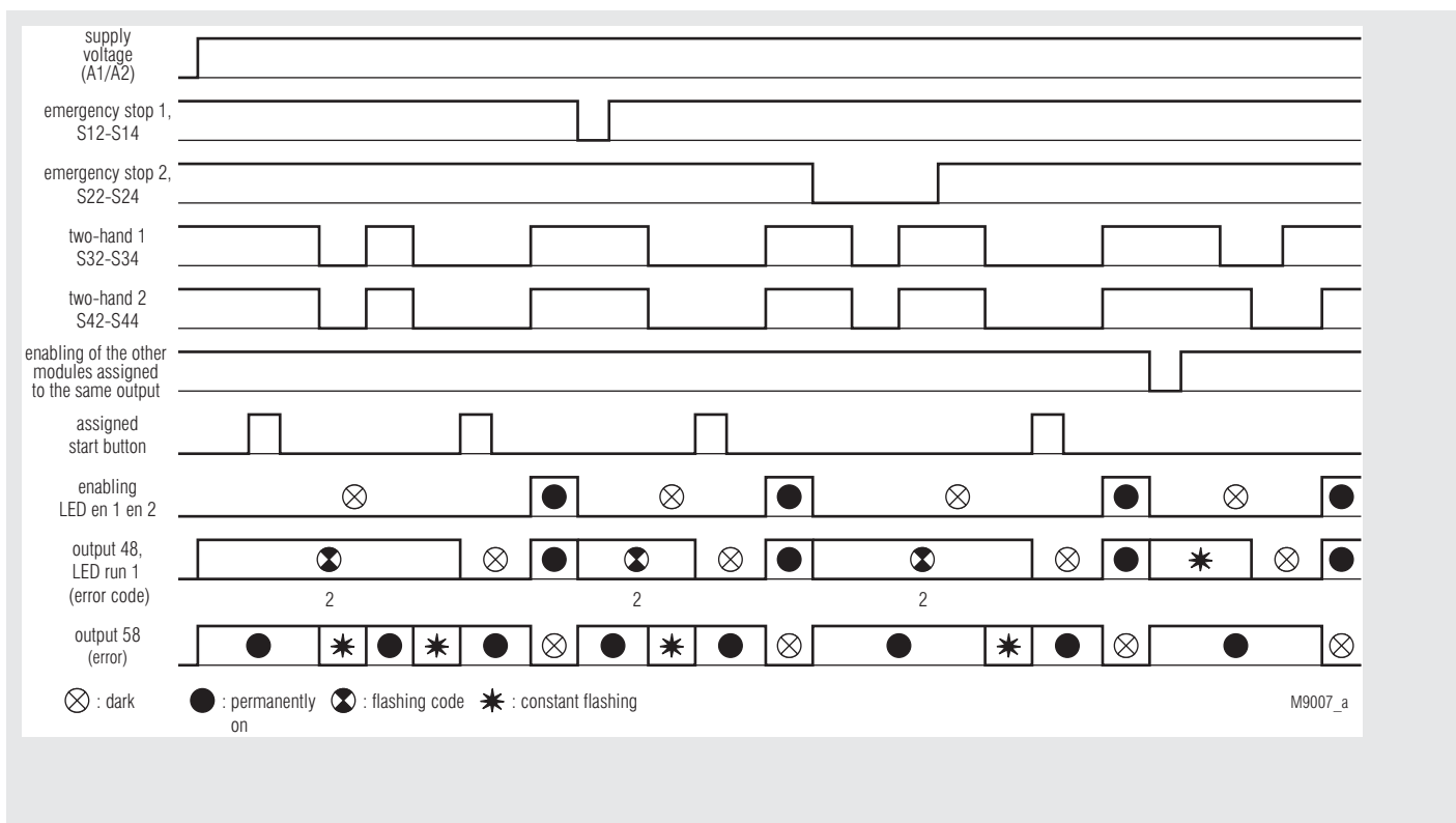
2 Emergency stop, manual start, 1 two-hand control type IIIC; function: 7 or 9
