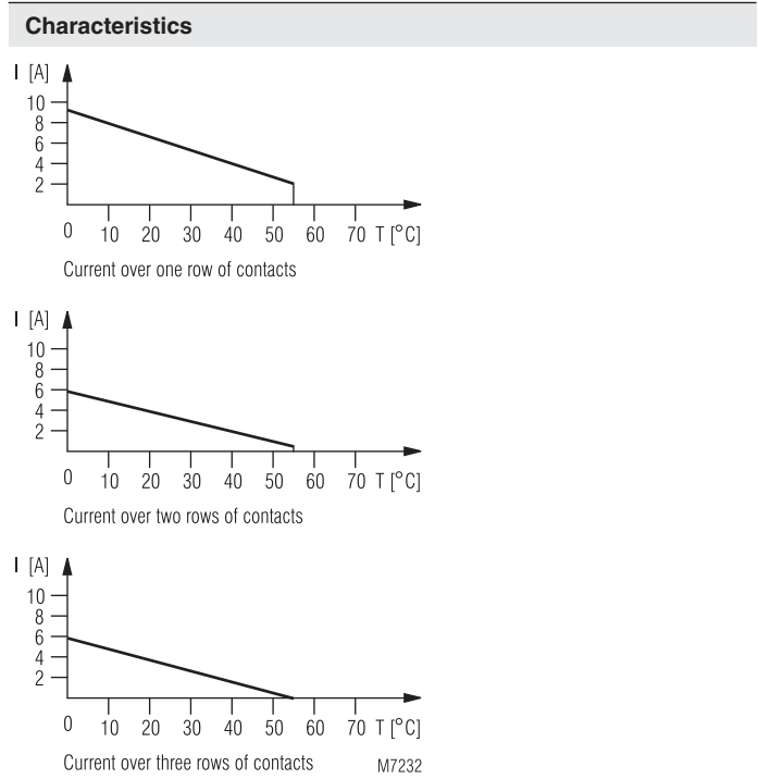
Continuous current limit curves as a function of ambient temperature
