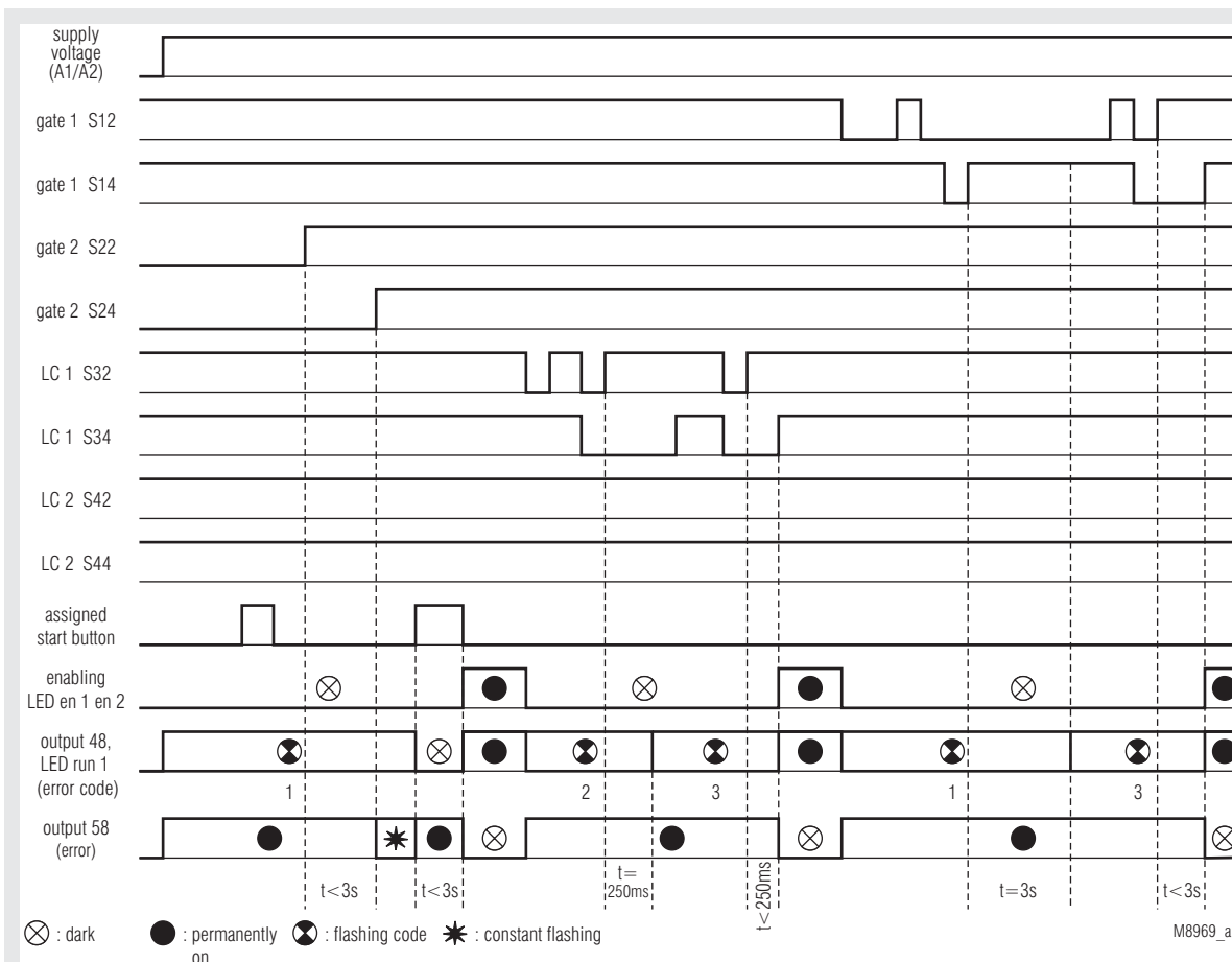
2 safety gates, 2 light curtains (Autostart)
