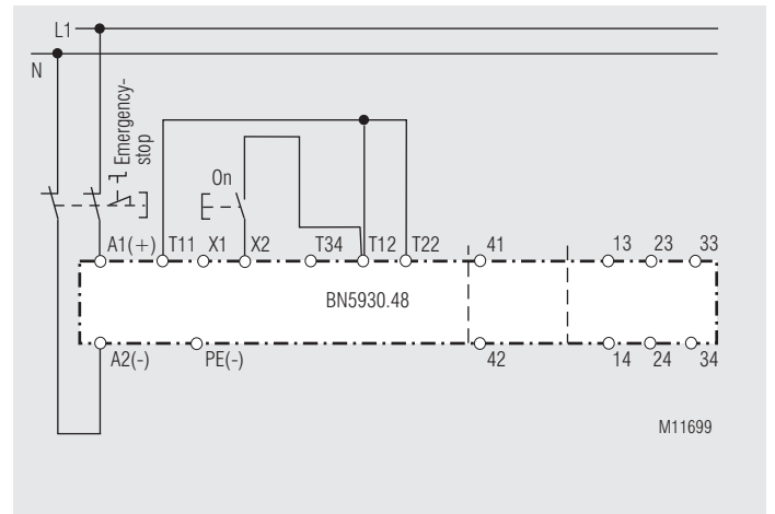
Two-pole emergency-stop with emergency-stop control device in the supply circuit.. Application for long emergency-stop loops in which the control voltage dropped below the minimum voltage of 21 V.
