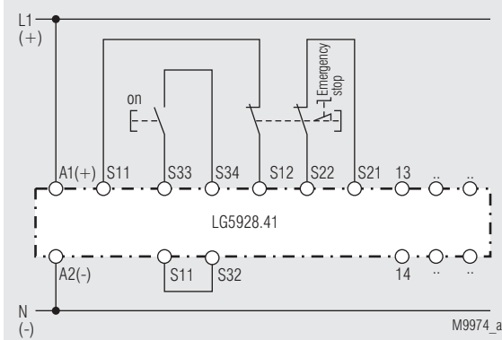
2-channel emergency stop circuit with cross fault monitoring. Suited up to SIL3, Performance Level e, Cat. 4
