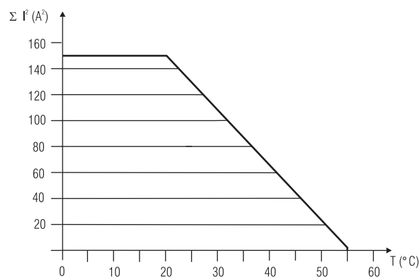
Arc limit curve for resistive load (delayed contact)
