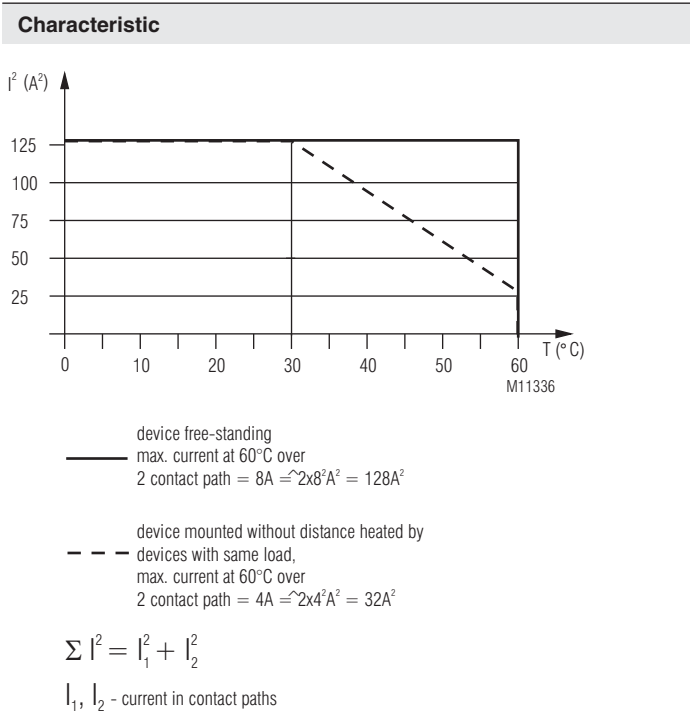
Quadratic total current limit curve
