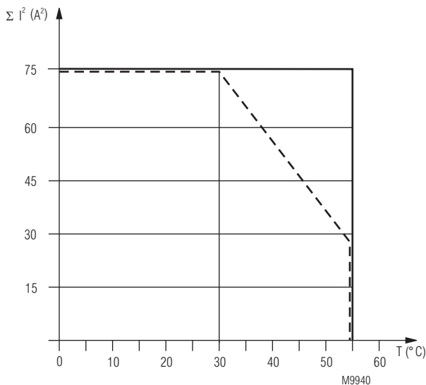
Total current limit curve BG 7925
