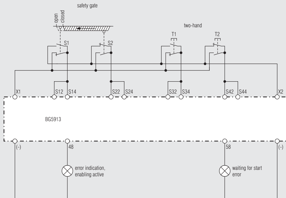
BG 5913.08/_2_ __, 1 safety gate, 1 two-hand control type IIIC (EN 574); function: 8
