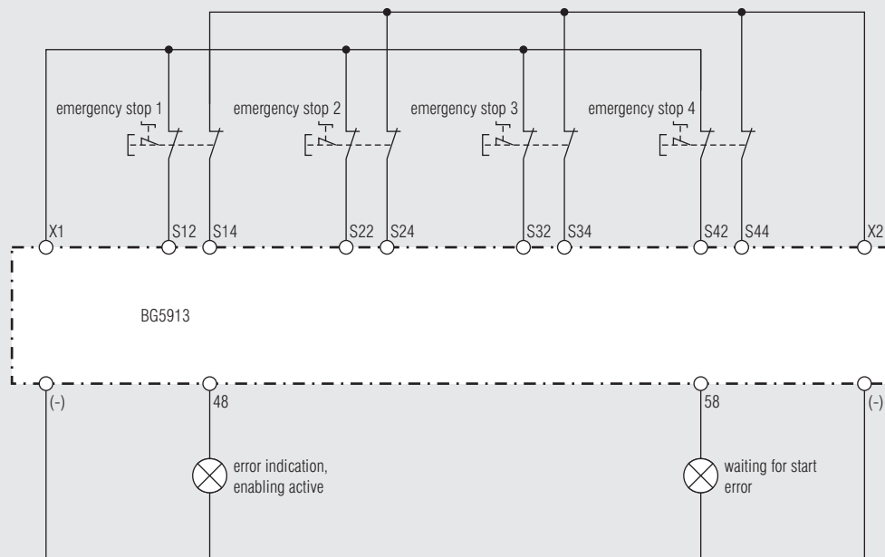
4 Emergency stop circuits, 2-channel, auto/manual start with short circuit monitoring; function: 0, 2
