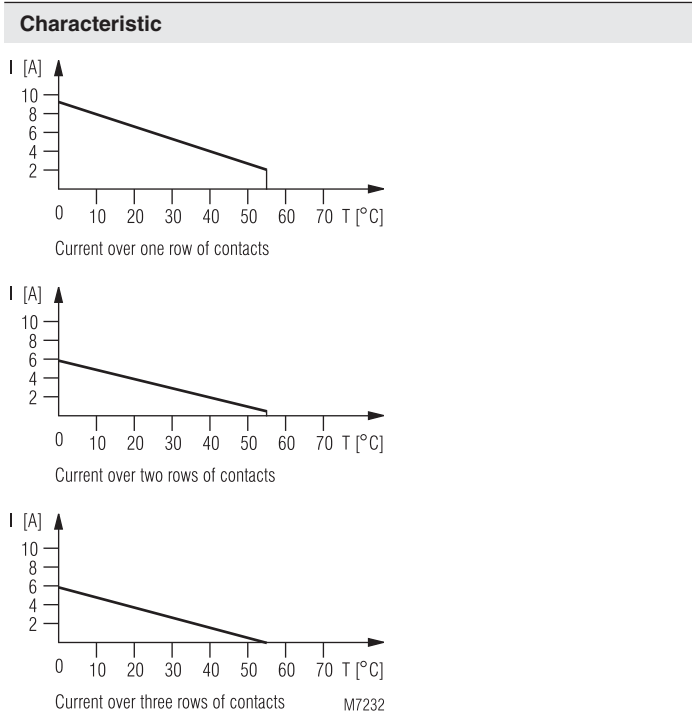
Continuous current limit curves depend on the ambient temperature
