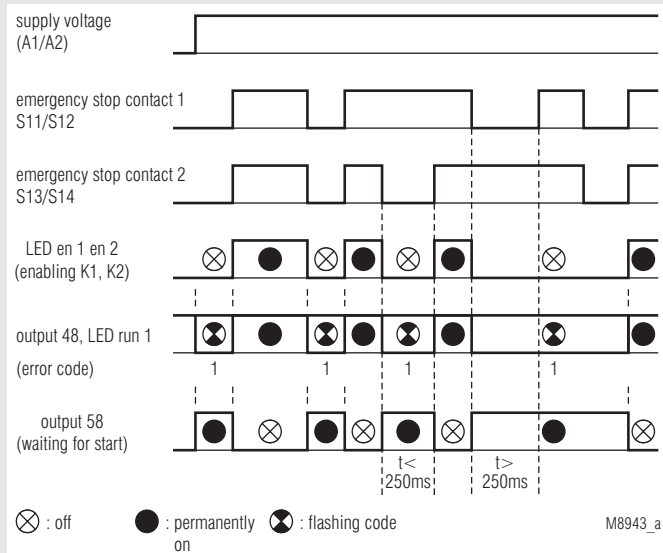
Emergency stop or light curtain, automatic start
