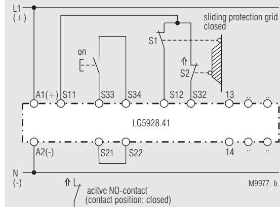
2-channel safety gate monitoring. Suited up to SIL3, Performance Level e, Cat. 4
