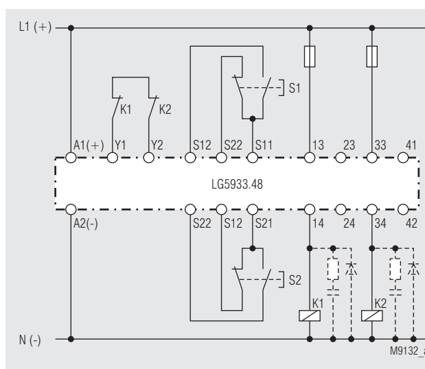
Two-hand control with contact reinforcement via external forcibly guided contactors. When switching inductive loads spark absorbers are recommended. Suited up to SIL3, Performance Level e, Cat. 4
