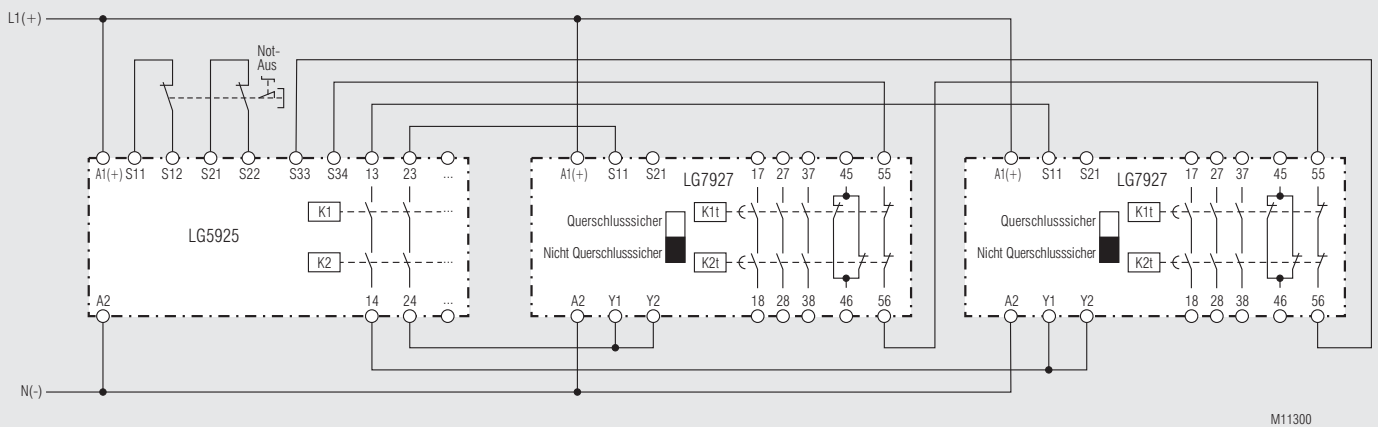
LG 5925 with two LG 7928, non cross fault detection, suitable up to SIL2, Performance Level d, Cat. 3
