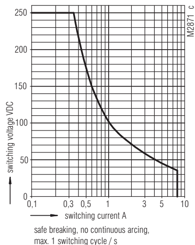
Limit curve for arc-free operation with resistive load (delayed contacts)
