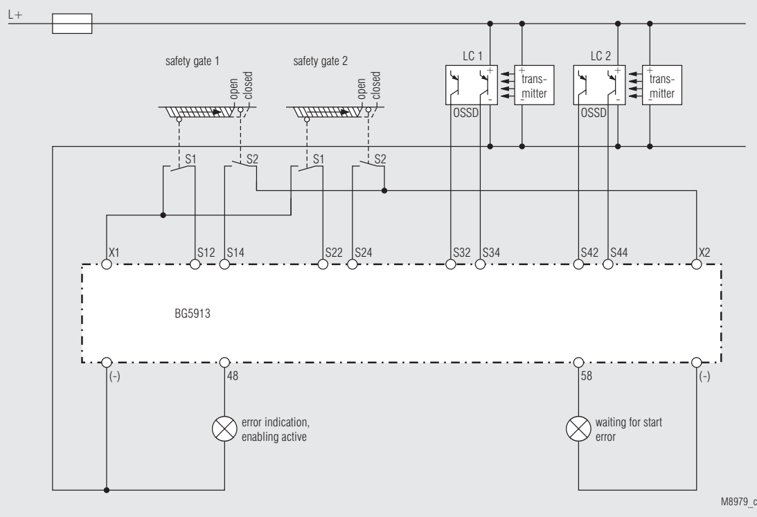
BG 5913.08/_1_ __, 2 safety gates, 2 light curtains; functions: 2 or 3
