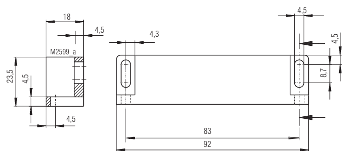
Transmitter
