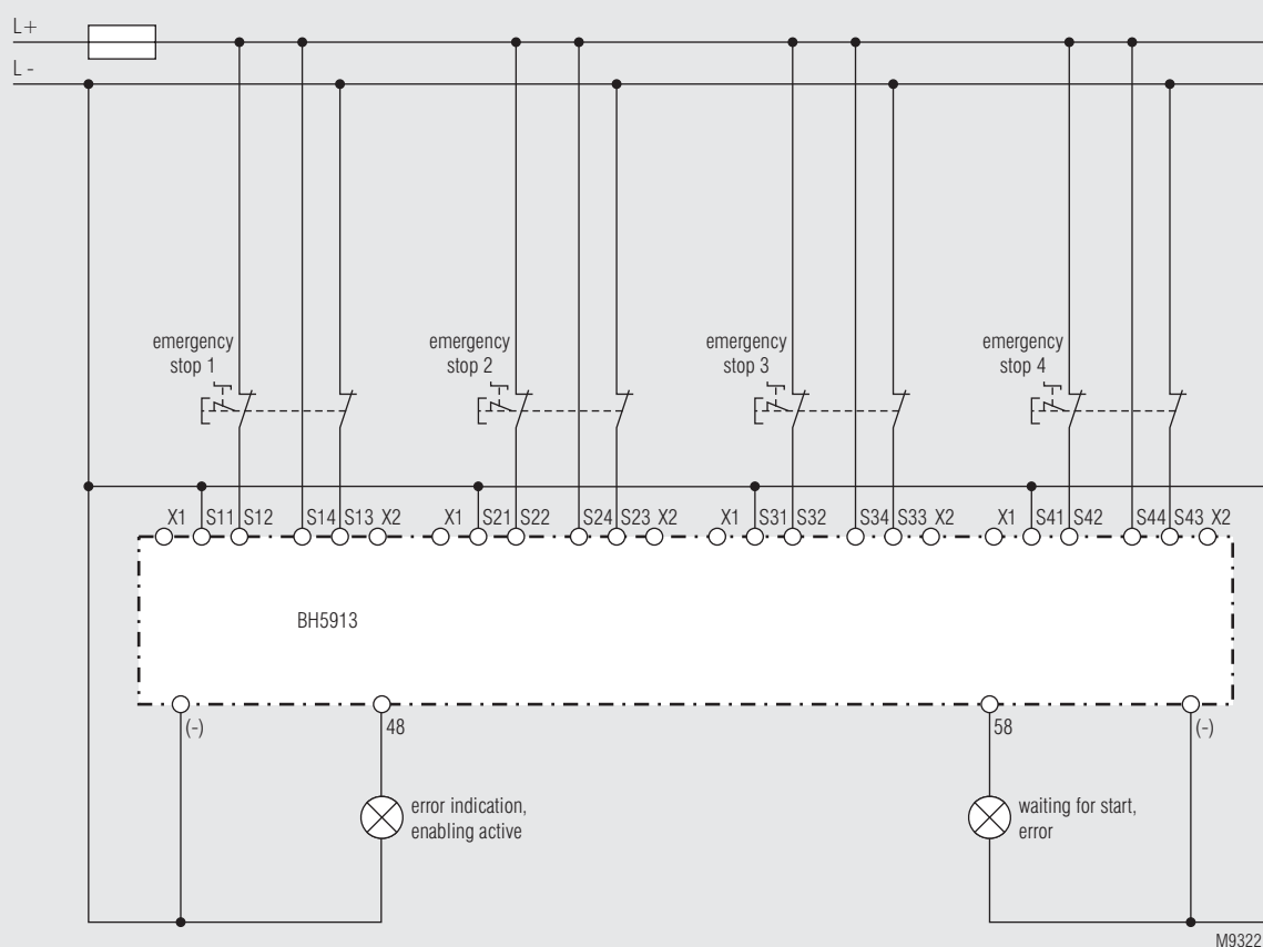
4 Emergency stop circuits, 2-channel, auto/manual start, short circuit monitoring by wiring; function 1, 3
