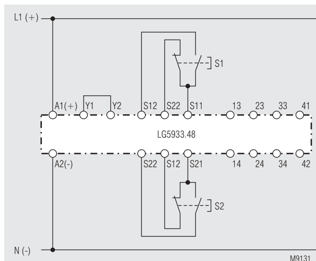
Two-hand control Suited up to SIL3, Performance Level e, Cat. 4
