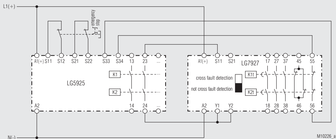
LG 5925 with LG 7927, non cross fault detection, suitable up to SIL2, Performance Level d, Cat. 3
