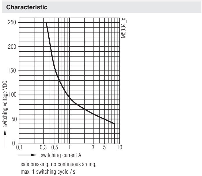
Arc limit curve under resistive load
