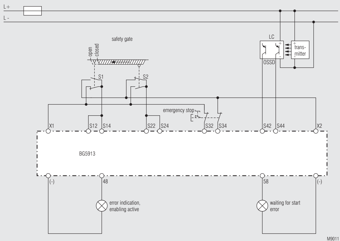
BG 5913.08/_2_ __, 1 safety gate, 1 Emergency stop, 1 light curtain; functions: 0 or 1
