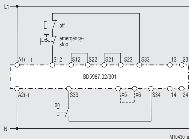
Single-channel emergency stop circuit. This circuit does not have any redundancy in the emergency stop control circuit. Suited up to SIL2, Performance Level d, Cat. 3
