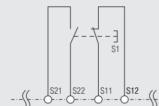
Fct.: Exclusive or contacts (5), with cross fault detection SIL 3, PL e, Cat. 4
