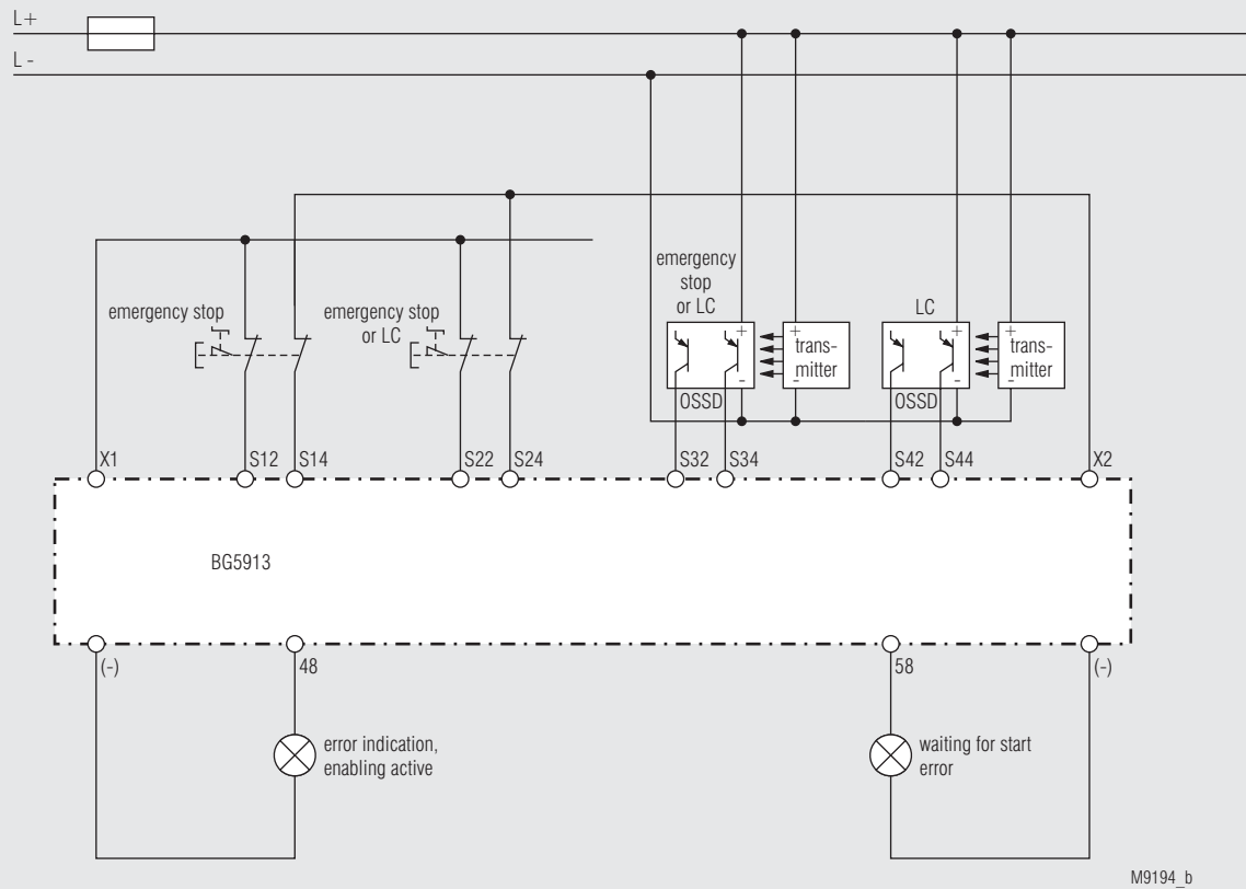
Emergency stop or light curtains; functions: 0, 1, 2, 3, 4 or 5
