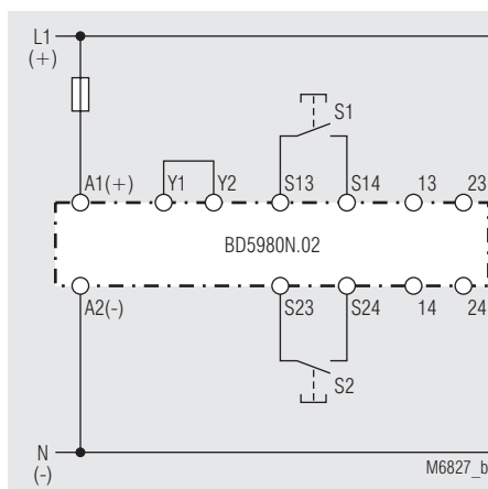
Two-hand control Suited up to SIL1, Performance Level c, Cat. 1
