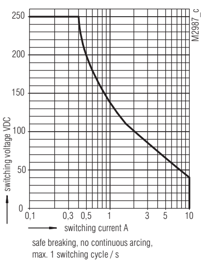
Limit curve for arc-free operation
