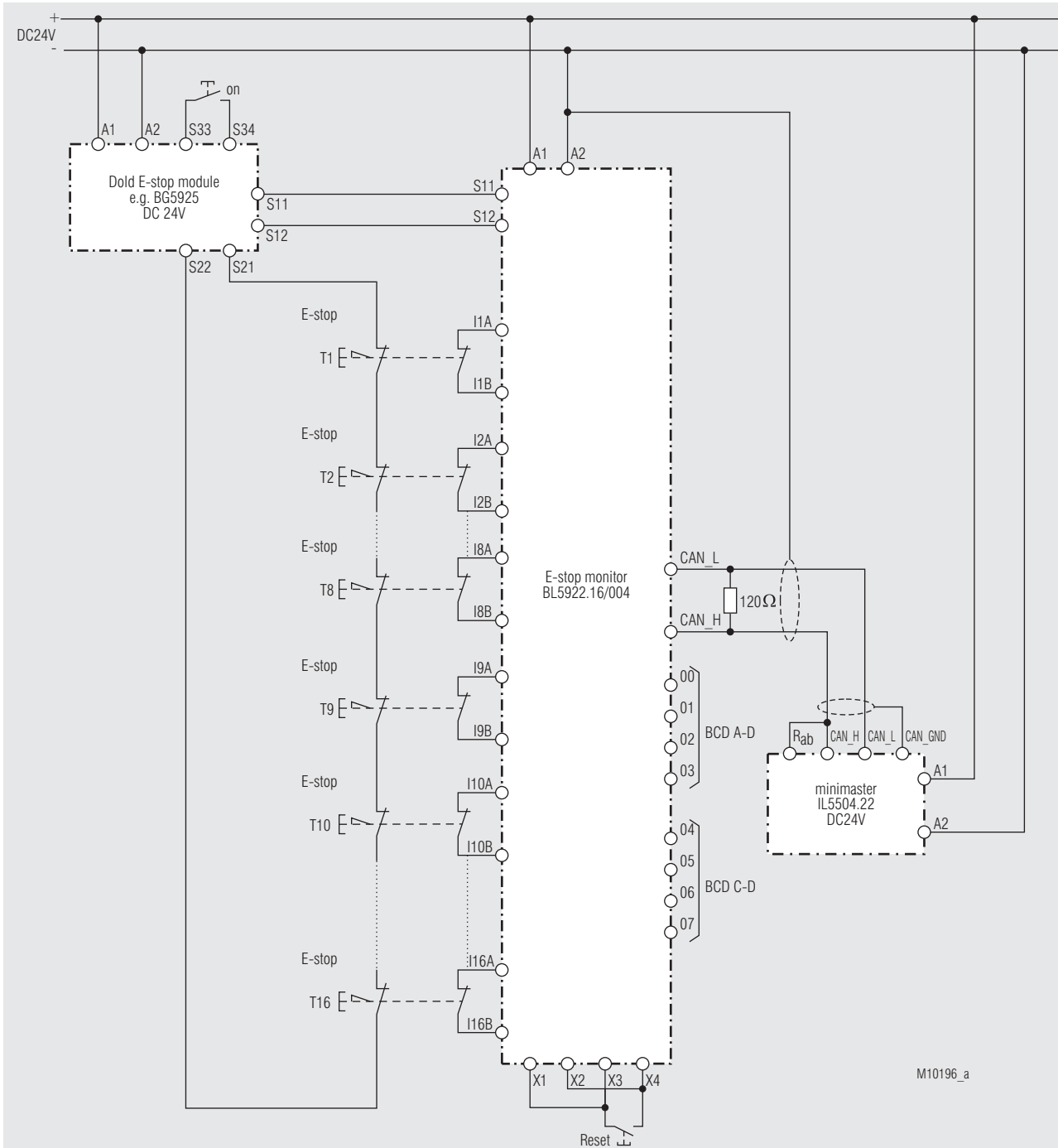
Pic 10: Monitoring of 16 e-stop buttons with e-stop monitor, single-channel connection, e-stop-module 2-channel, cross fault monitoring. BCD-output for remote display of the status of the e-stop buttons.
