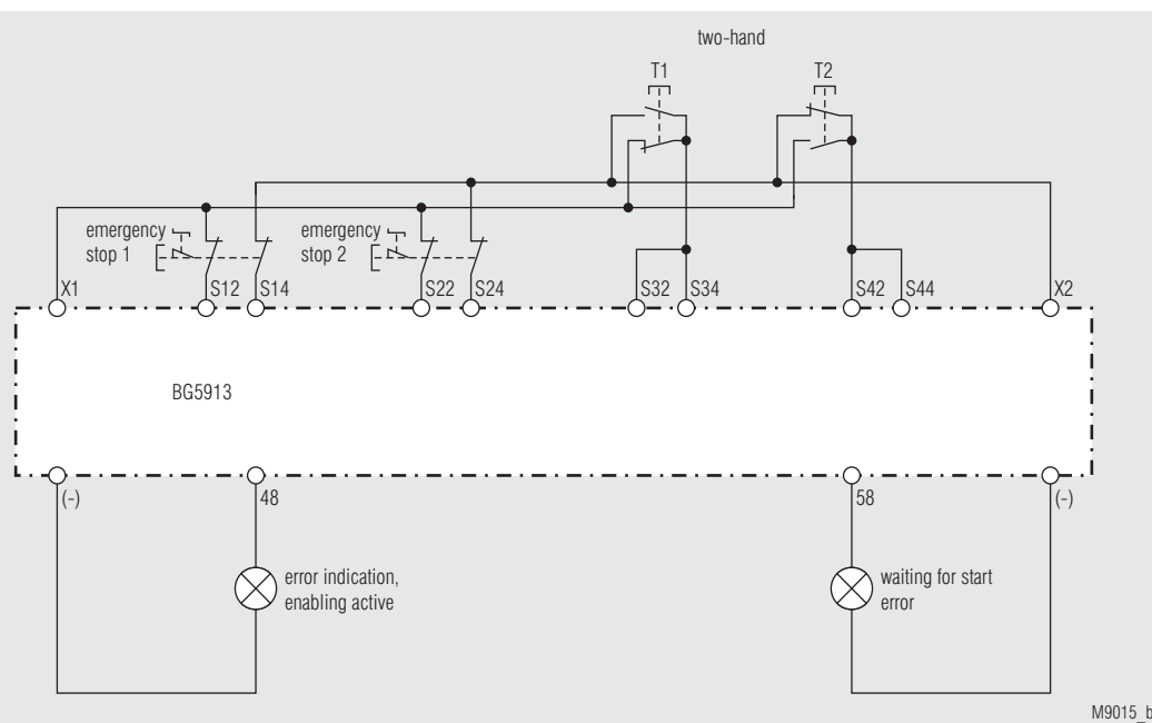
BG 5913.08/_2_ ___, 4 Emergency stop; functions: 2, 3, 4 or 5
