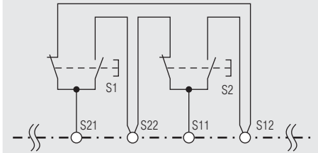
Fct.: Two-hand control (3), with cross fault detection SIL 3, PL e, Cat. 4 Type III C to EN 574
