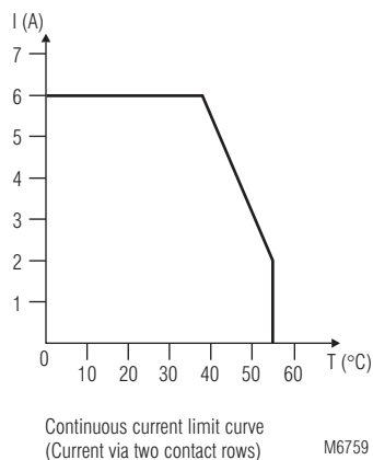
Continuous current limit curve
