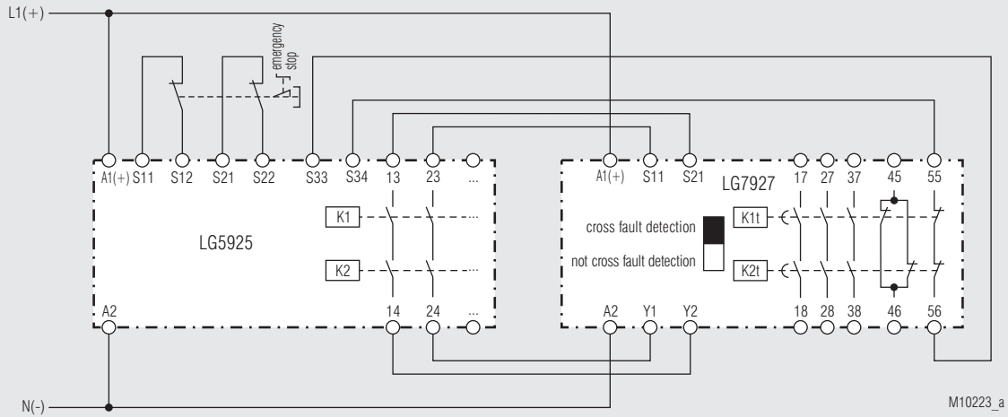
LG 5925 with LG 7928, cross fault detection, suitable up to SIL2, Performance Level d, Cat. 3
