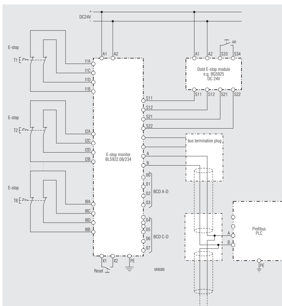
Pic 9: Monitoring of 8 e-stop buttons with e-stop monitor, 2-channel connection, 2-channel monitoring cross fault monitoring with Profibus DP-PLC
