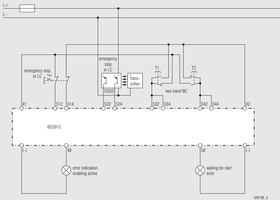
Emergency stop or light curtains, two-hand control type IIIC; functions 6, 7, 8 or 9
