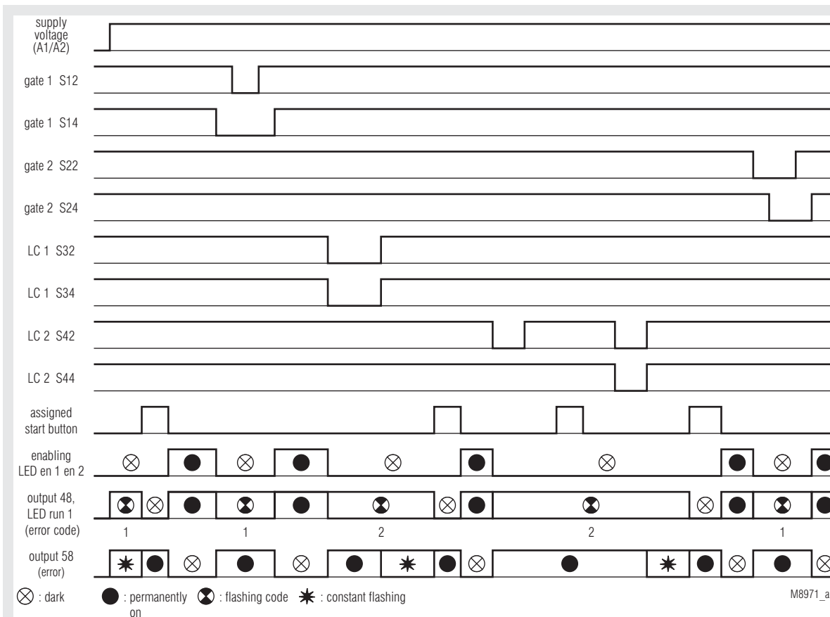
2 safety gates, 2 light curtains (manual start)
