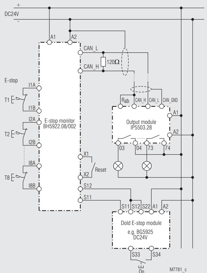
Pic 2: Monitoring of 8 e-stop buttons with e-stop monitor, single-channel connection, e-stop module 2-channel. Remote display of the status of e-stop buttons via CANopen interface.
