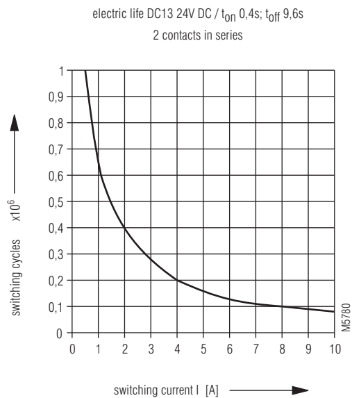
Contact service life
