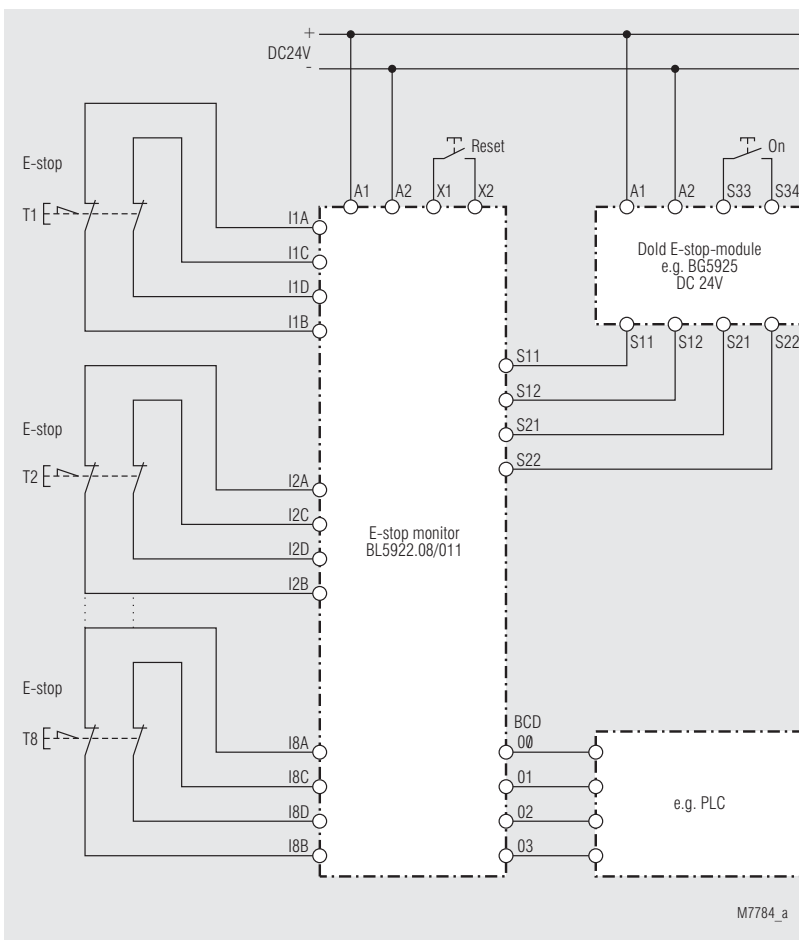
Pic 5: Monitoring of 8 e-stop buttons with e-stop monitor, 2-channel connection, BCD output, single-channel monitoring
