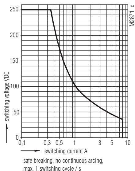
Arc limit curve for resistive load (delayed contact)
