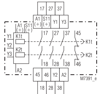
BG 7925.96/002, BG 7925.96/003 2 timing circuits
