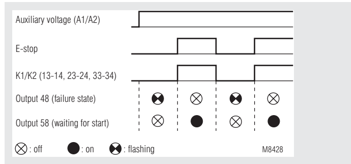
E-stop, 2-channel, auto start
