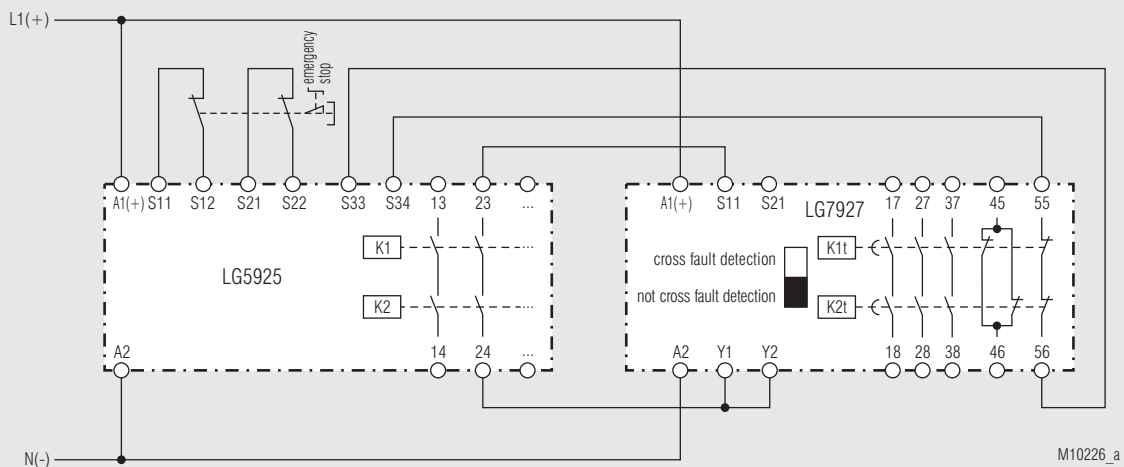
LG 5925 with LG 7928, non cross fault detection, suitable up to SIL2, Performance Level d, Cat. 3
