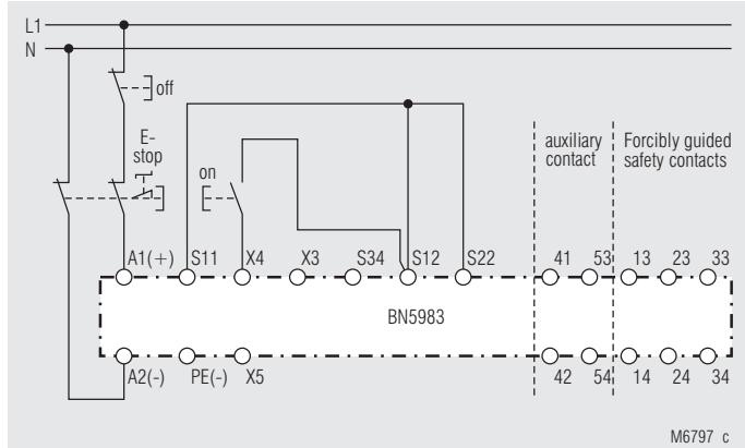
Two-pole emergency-stop circuit with emergency stop control device in supply circuit. Application for long emergency stop loops where the control voltage drops below the minimum voltage of 21 V. Attention: Single faults (e.g. line faults at the emergency stop control device) are not detected with this external circuit configuration. Suited up to SIL3, Performance Level e, Cat. 4
