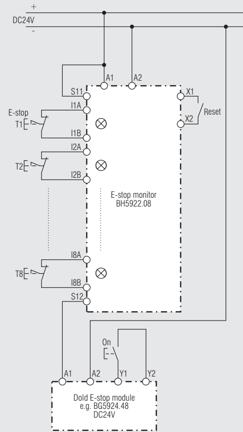
Pic 1: Monitoring of 8 e-stop buttons with e-stop monitor, single-channel connection, e-stop module single channel. Display via 8 LEDs on frontside of the module
