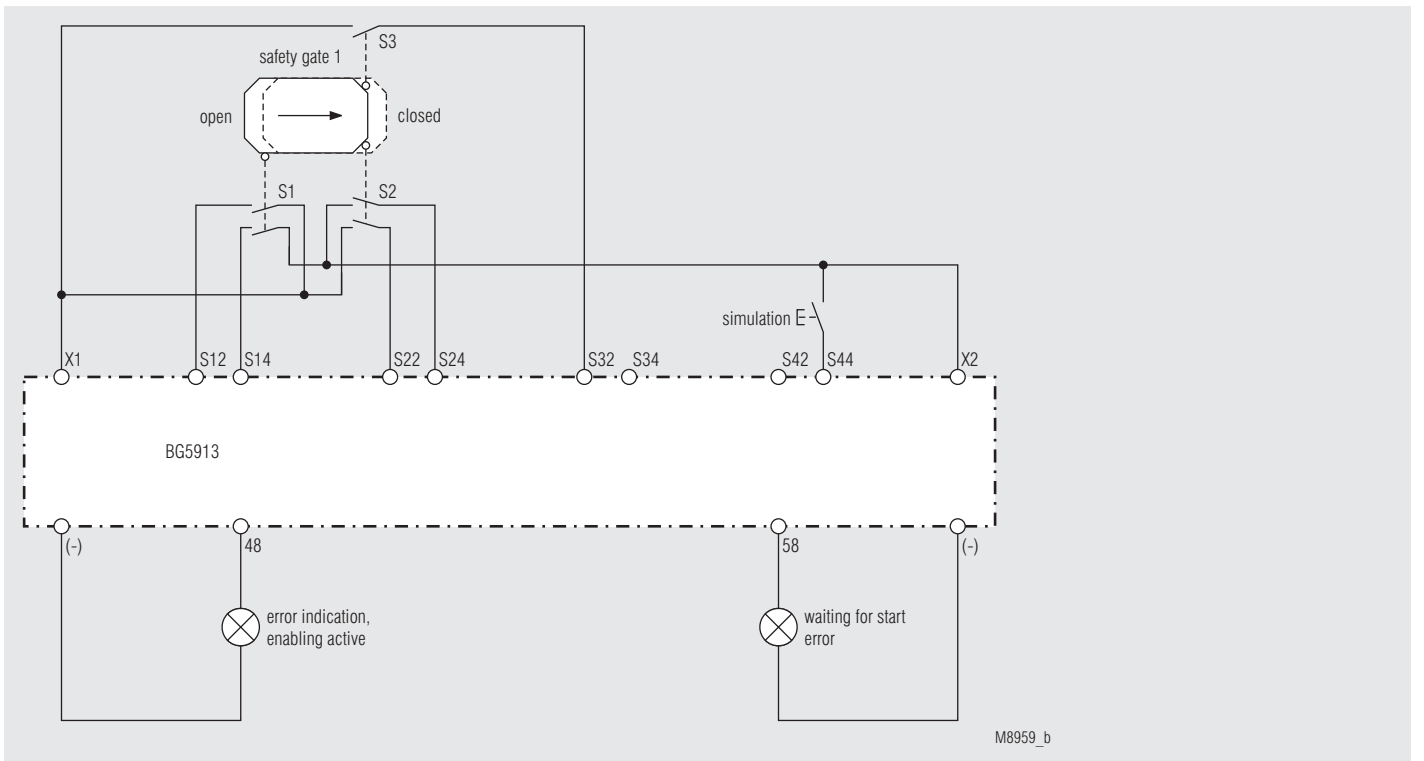
1 safety gate with 2 twin/1 single contact, manual start (plastic injection moulding machines); function: 6
