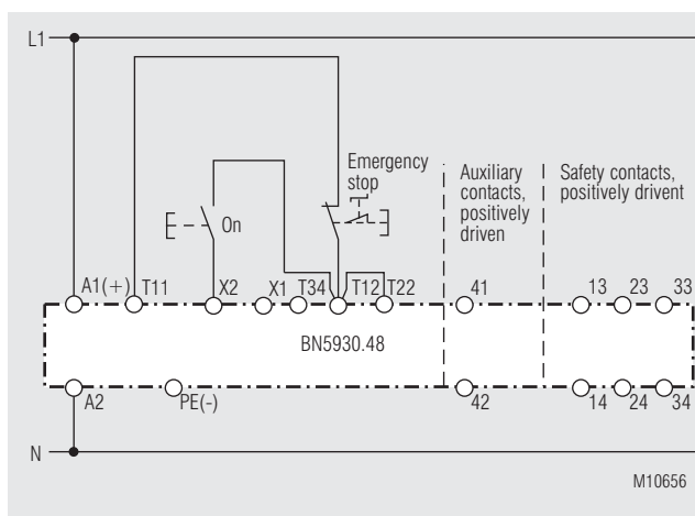
One-channel emergency-stop circuit. This circuit does not have any redundancy in the emergency-stop control circuit. Suited up to SIL2, Performance Level d, Cat. 3
