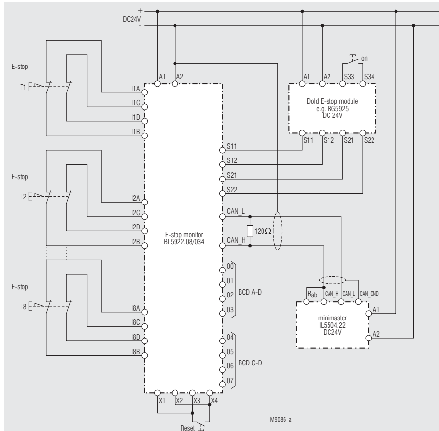
Pic 8: Monitoring of 8 e-stop buttons with e-stop monitor, 2-channel connection, 2-channel monitoring cross fault monitoring with CANopen minimaster IL 5504, IN 5504
