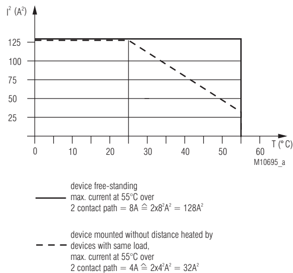
UG 6980.04 Quadratic total current limit curve
