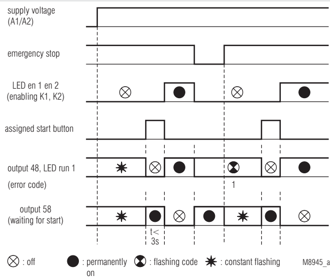
Emergency stop or light curtain, manual start
