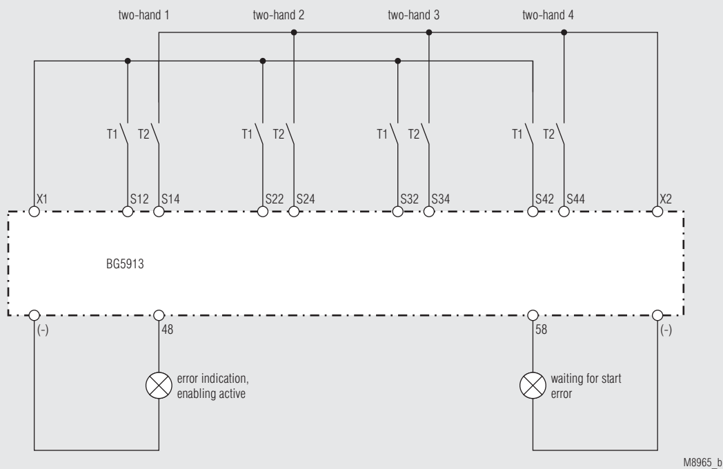
4 two-hand controls type IIIA acc. to DIN/EN 574; function: 8
