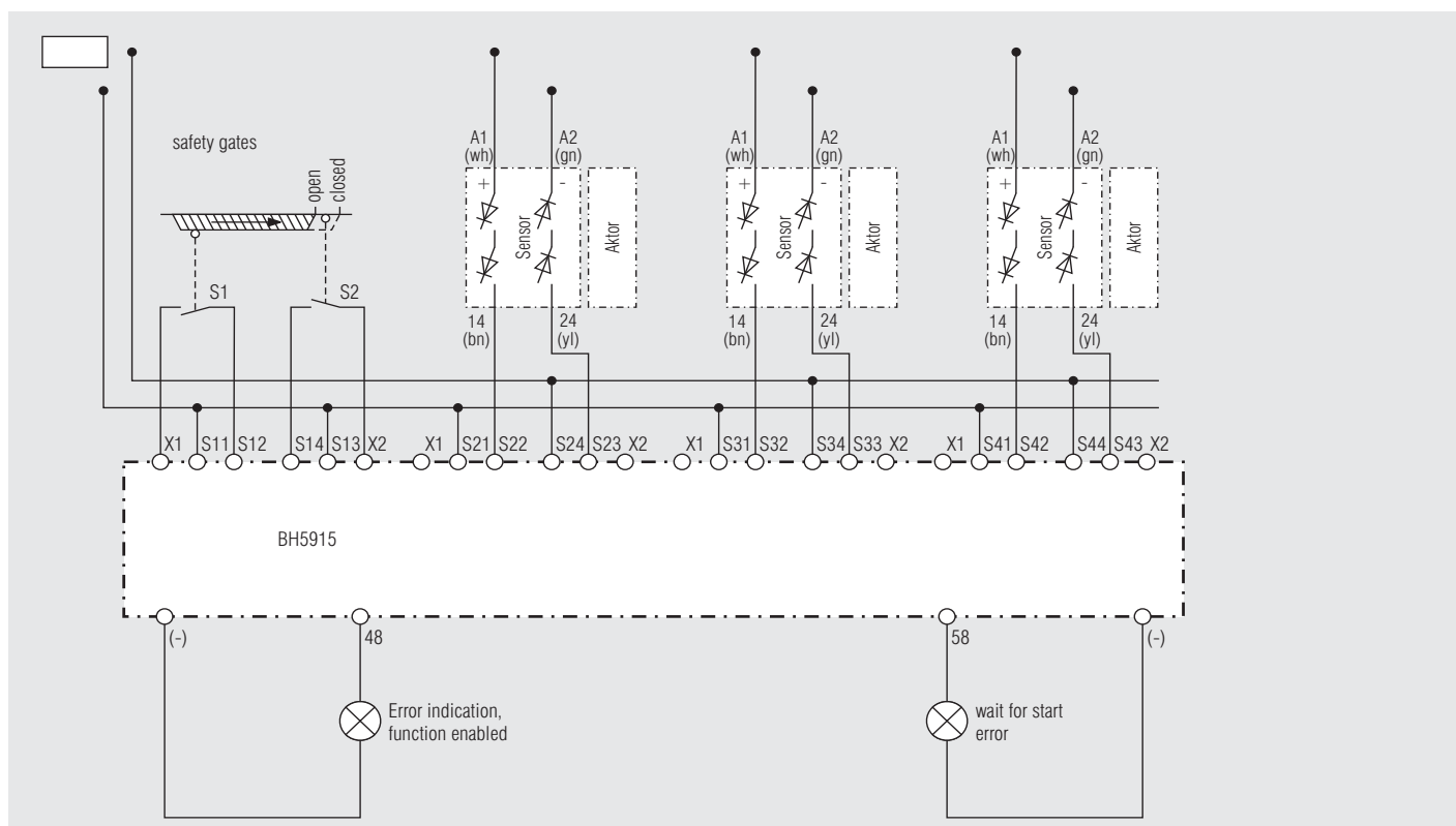
BH 5915.08/01MF0, Connection at sensors with semiconductor outputs
