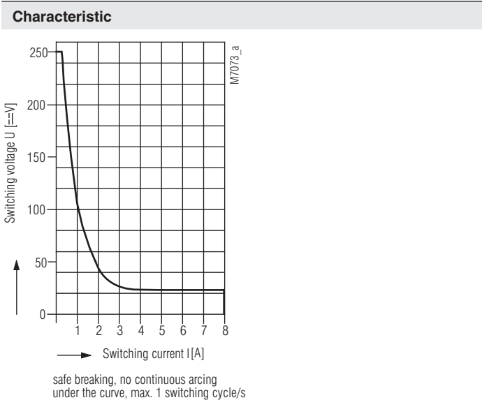
Arc limit curve
