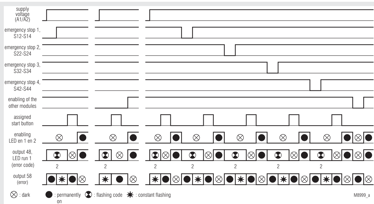
4 Emergency stop, Autostart, only enabling when all the other modules are enabled; function: 2
